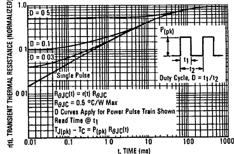
FIGURE 31 — THERMAL RESPONSE
