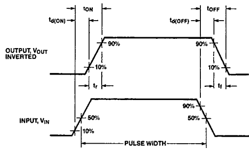
Figure 12 Switching Waveforms
