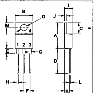
TO-220
