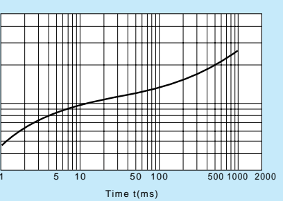
θ j-a -t Characteristics
