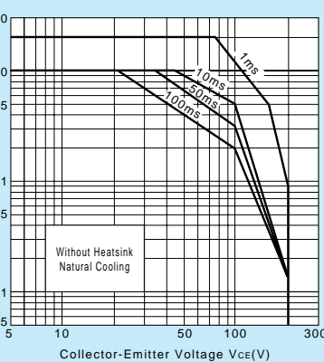
Safe Operating Area (Single Pulse)
