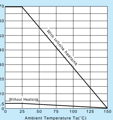
P C -T a Derating
