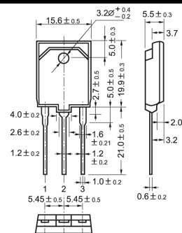
TO-3PFM
