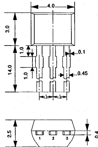
OUTLINE DRAWING
