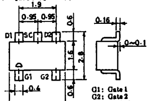
Case Outline—[2070] unit: mm
