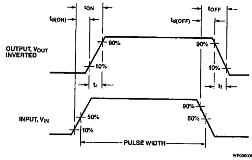
Figure 10 Switching Waveforms
