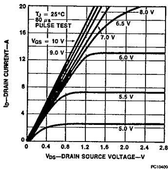
Figure 1 Output Characteristics
