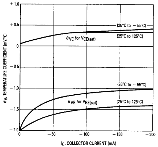
FIGURE 12 — TEMPERATURE COEFFICIENTS
