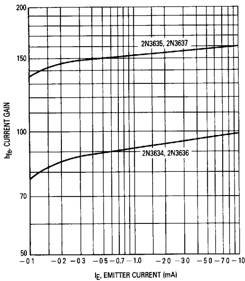
FIGURE 9 — CURRENT GAIN
