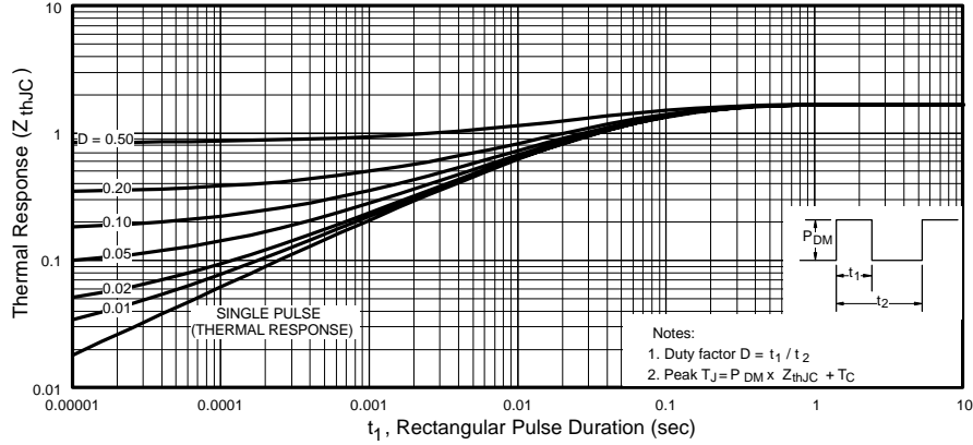
Fig. 4 - Max. Thermal Impedance Z_{thJC} Characteristics (Per Leg)
