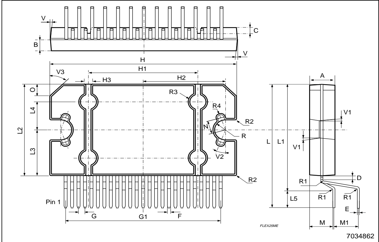
Flexiwatt25 (vertical)
