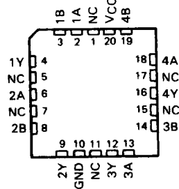
SN54F36 ... FK PACKAGE (TOP VIEW)
