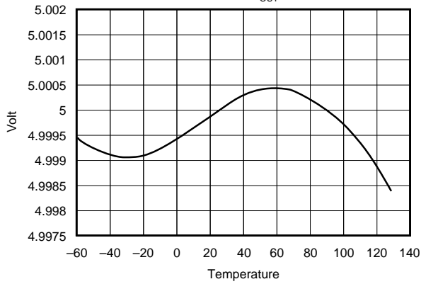
REF02 V_{OUT}
