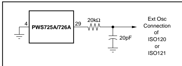
FIGURE 5. Synchronization with ISO120 or ISO121 Isolation Amplifier.
