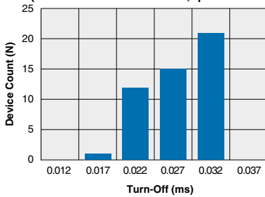
OAA160 Typical Turn-Off Time (N=50 Ambient Temperature = 25°C) (Load Current = 50mADC; I F = 10mADC)
