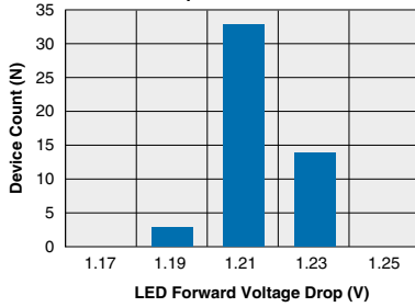
OAA160 Typical LED Forward Voltage Drop (N=50 Ambient Temperature = 25°C) I F = 10mADC
