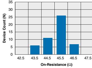
OAA160 Typical On-Resistance Distribution (N=50 Ambient Temperature = 25°C) (Load Current = 50mADC; I F = 10mADC)
