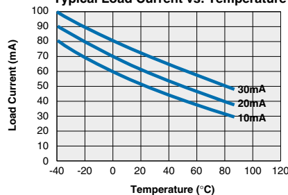
OAA160 Typical Load Current vs. Temperature
