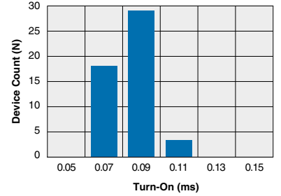
OAA160 Typical Turn-On Time (N=50 Ambient Temperature = 25°C) (Load Current = 50mADC; I F = 10mADC)
