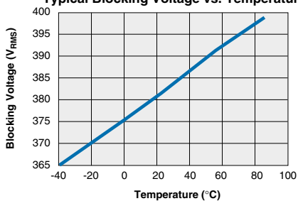
OAA160 Typical Blocking Voltage vs. Temperature
