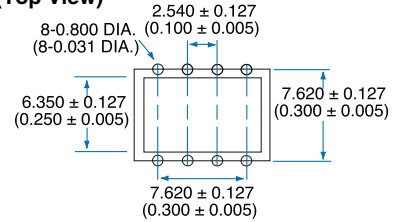
PC Board Pattern (Top View)
