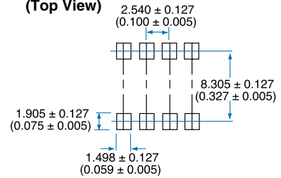
PC Board Pattern (Top View)
