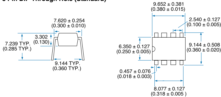
8 Pin DIP Through Hole (Standard)
