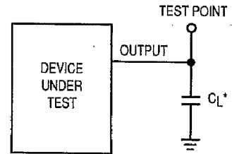
Figure 2. Test Circuit
