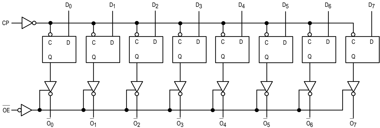
LOGIC DIAGRAM
