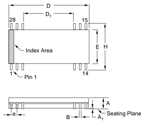
Package Number 217-2 — 28-Lead SOIC
