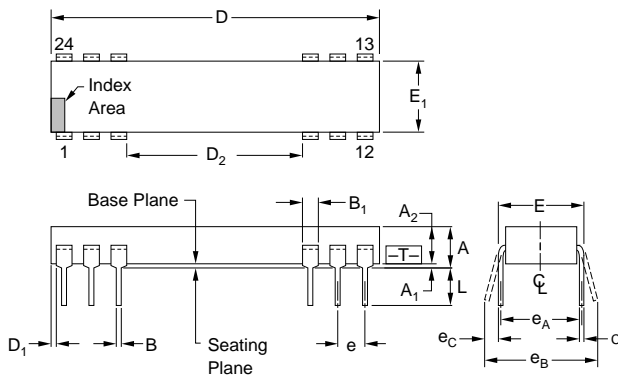
Package Number 243-1— 24-Lead Single-Wide PDIP
