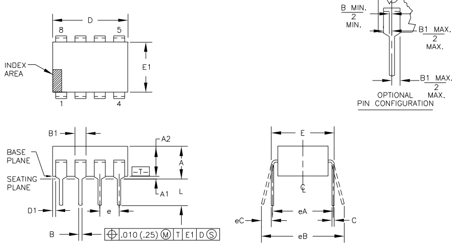
Package Number 006-3 - 8-Pin Plastic, Single-Wide DIP
