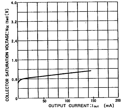
Fig. 6 Collector saturation voltage vs. output current
