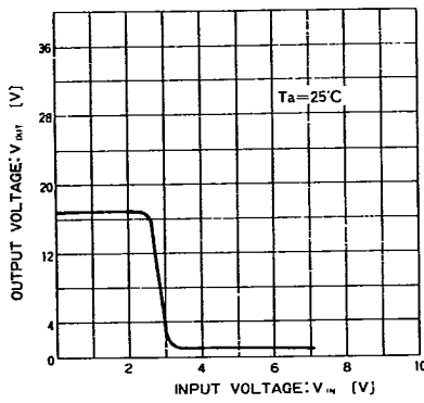
Fig. 7 Output voltage vs. input voltage
