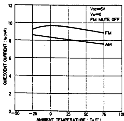
Fig. 11 Quiescent current vs. ambient temperature
