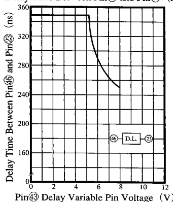
Delay Time Between Pin④⑥ and Pin③ (ns)
